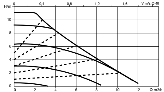
EVOPLUS B 110/250.40 M - EVOPLUS D 110/250.40 M
